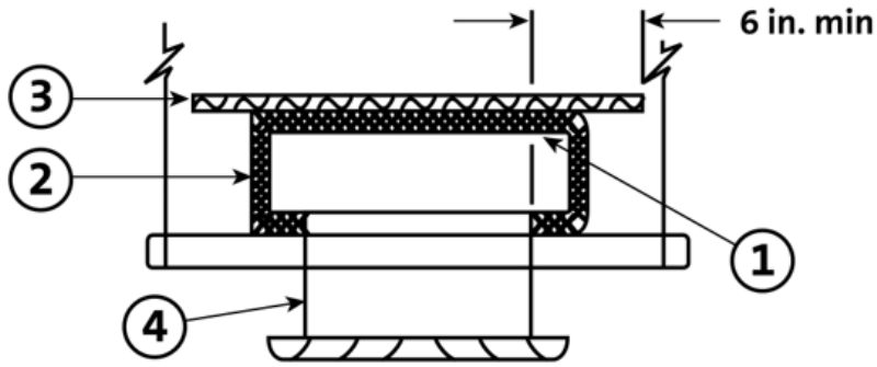
Transverse Cross-Section
