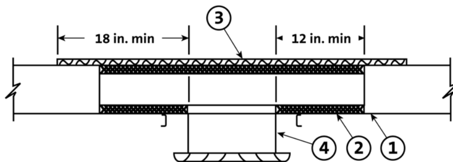
Longitudinal Cross-Section
