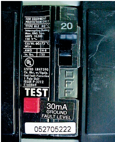
GFPE Circuit Breaker
